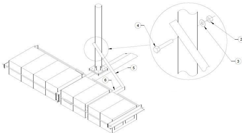
Brace Angle and Lower Mount Angle Assembly Figure 9
