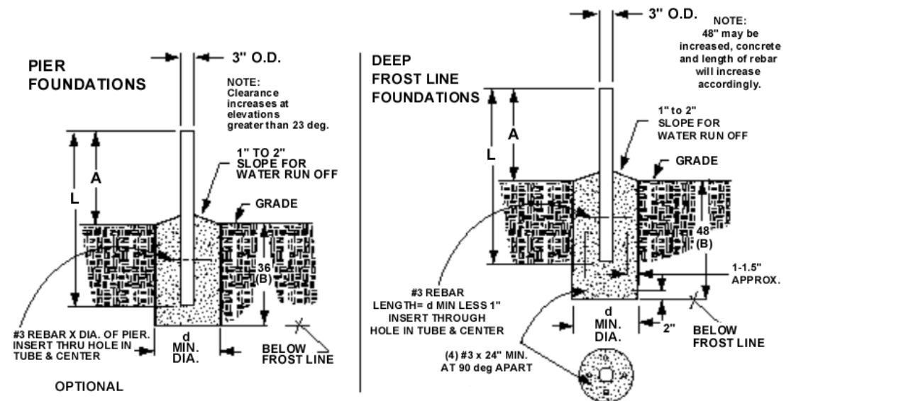
Foundation Diagram Figure 22
