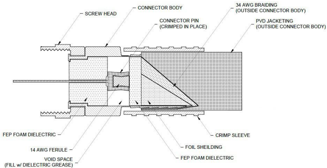
Crimping RG11 Cable Figure 37
