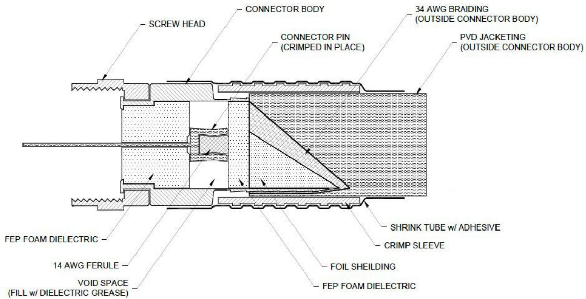
Weather Sealing RG11 Cable Figure 38
