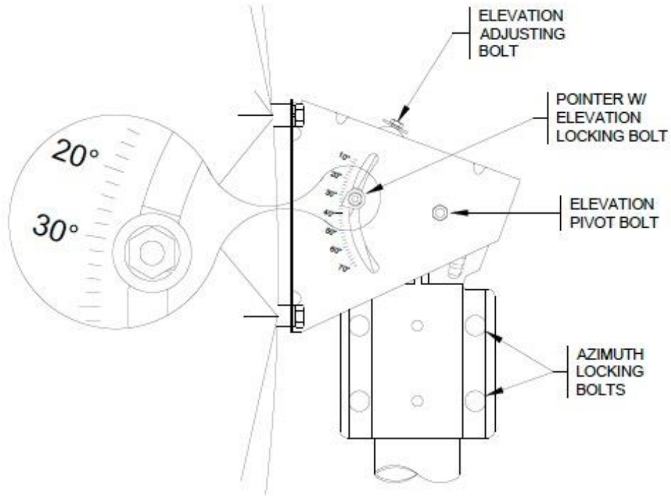
Elevation Adjustment Figure 34
