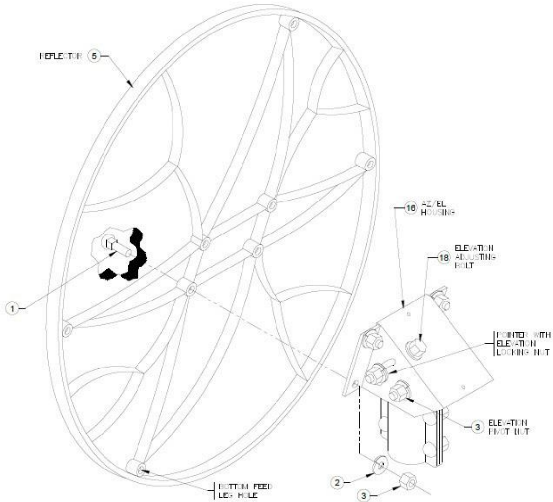
1.2-Meter Reflector Assembly Figure 24
