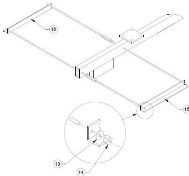
Angle Clamp Assembly Figure 5
