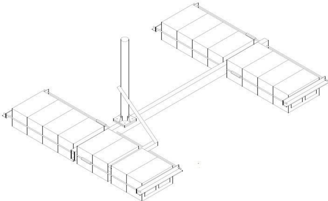
Mount Assembly Figure 1
