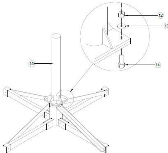
Mast Assembly Figure 20
